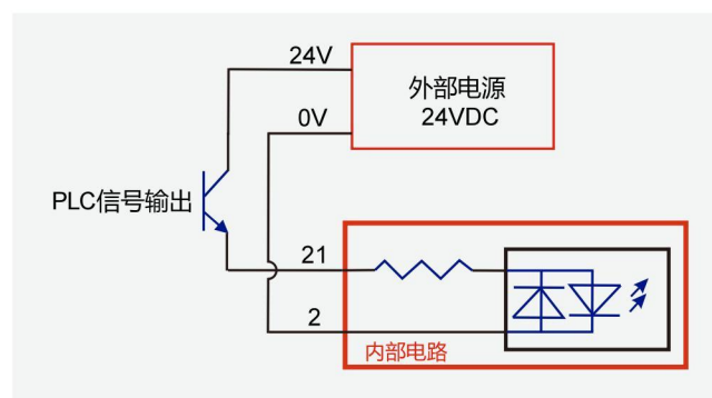
PNP
