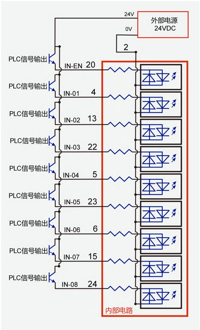
PNP
